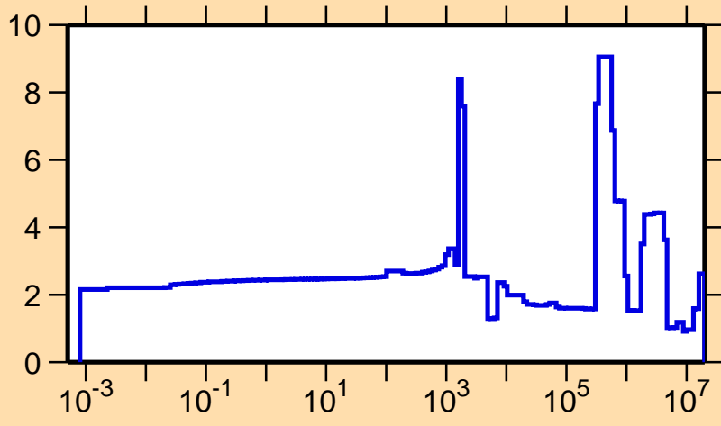
\Delta\sigma/\sigma vs. E for ^{122}\text{Sn}(n,\text{tot.})
