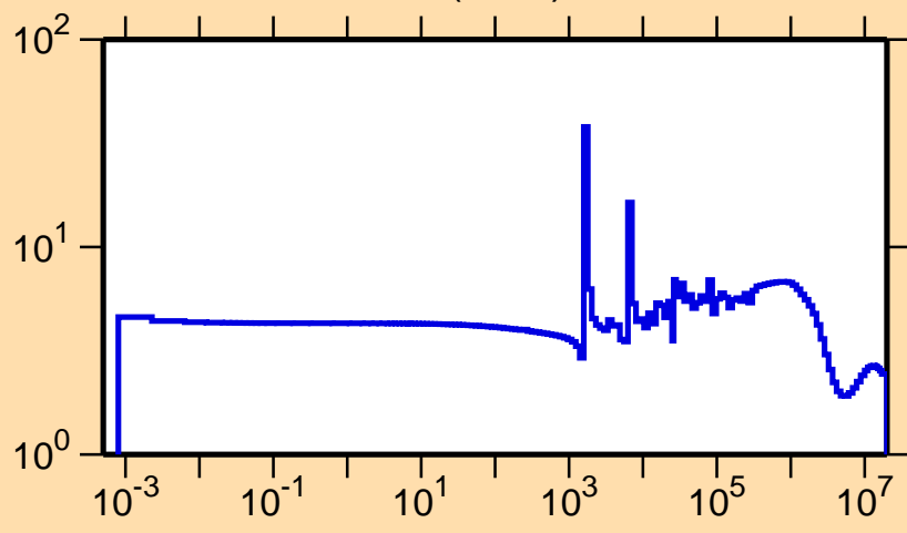
\sigma vs. E for ^{122}\text{Sn}(n,\text{el.})
