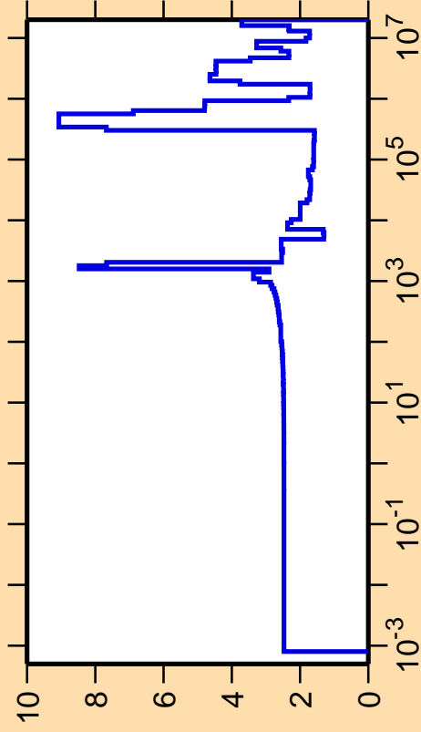
\Delta\sigma/\sigma vs. E for ^{122}\text{Sn}(n,\text{el.})
