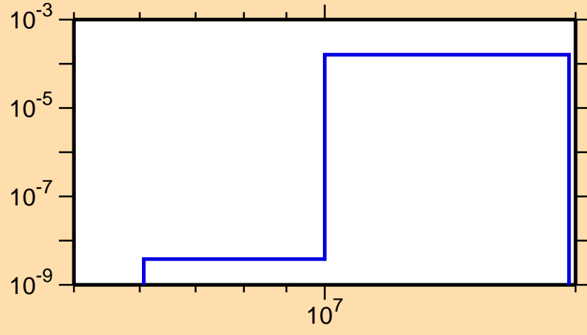
\sigma vs. E for ^{122}\text{Sn}(n,\alpha)
