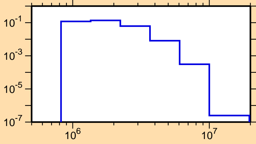
\sigma vs. E for ^{123}\text{Sn}(n,n_4)
