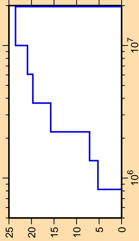
\Delta\sigma/\sigma vs. E for ^{123}\text{Sn}(n,n_4)
