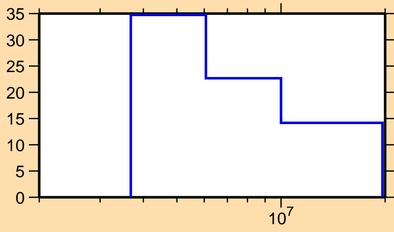
\Delta\sigma/\sigma vs. E for ^{123}\text{Sn}(n,\gamma)
