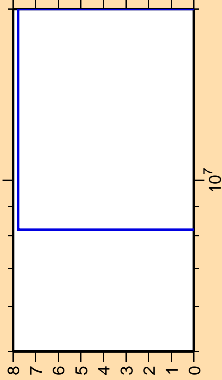
\Delta\sigma/\sigma vs. E for ^{123}\text{Sn}(n,3n)
