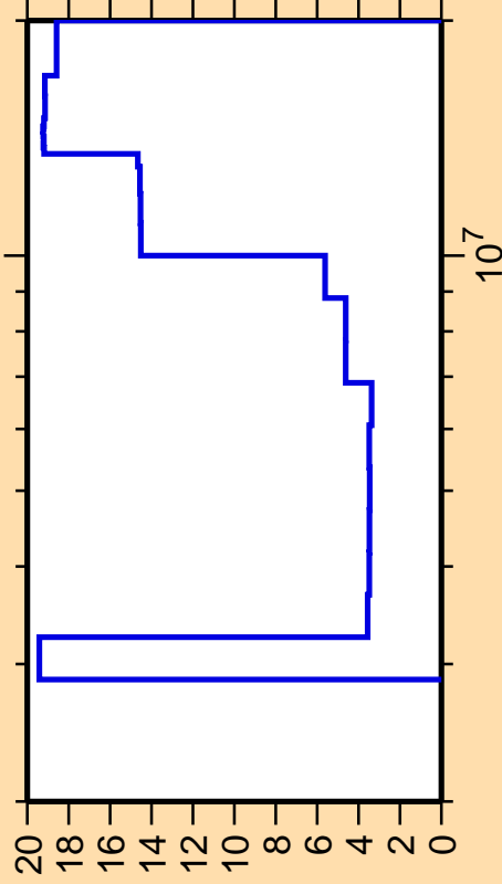
\Delta\sigma/\sigma vs. E for ^{124}\text{Sn}(n,n\text{cont.})
