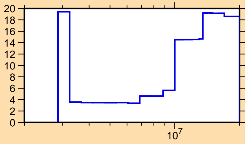
\Delta\sigma/\sigma vs. E for ^{124}\text{Sn}(n,n\text{cont.})
