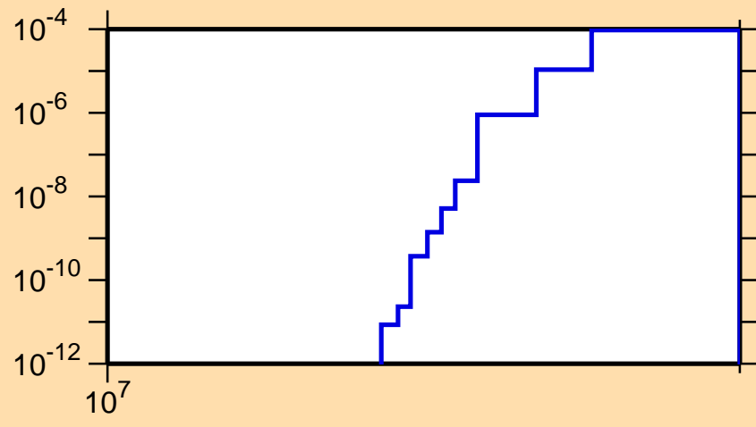
\sigma vs. E for ^{124}\text{Sn}(n,np)
