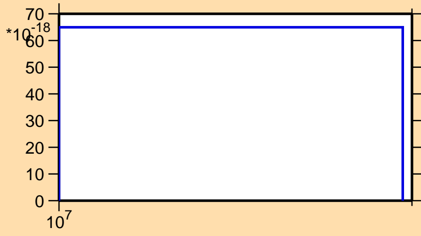
\sigma vs. E for ^{124}\text{Sn}(n,\text{nd})
