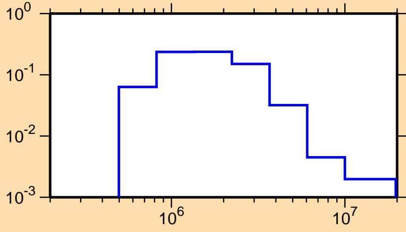
\sigma vs. E for ^{125}\text{Sn}(n,n_3)
