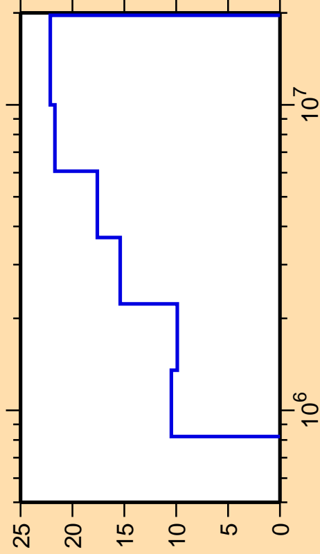
\Delta\sigma/\sigma vs. E for ^{125}\text{Sn}(n,n_4)
