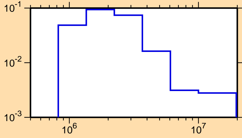
\sigma vs. E for ^{125}\text{Sn}(n,n_4)
