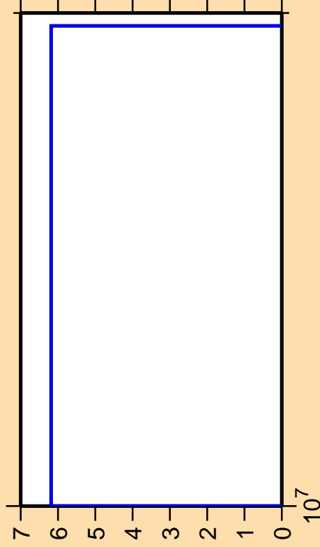
\Delta\sigma/\sigma vs. E for ^{125}\text{Sn}(n,\text{nd})
