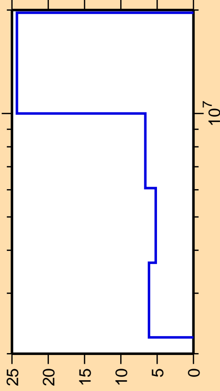
\Delta\sigma/\sigma vs. E for ^{125}\text{Sn}(n,n\text{cont.})
