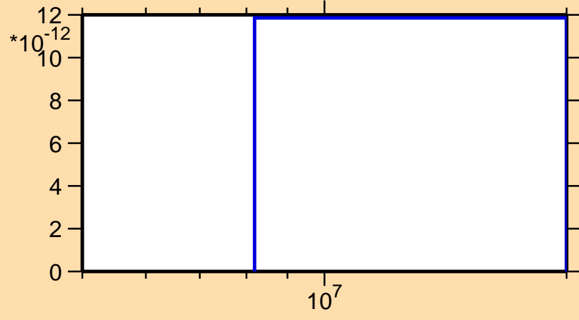
\sigma vs. E for ^{125}\text{Sn}(n,nd)
