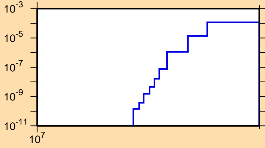
\sigma vs. E for ^{127}\text{Sn}(n,d)
