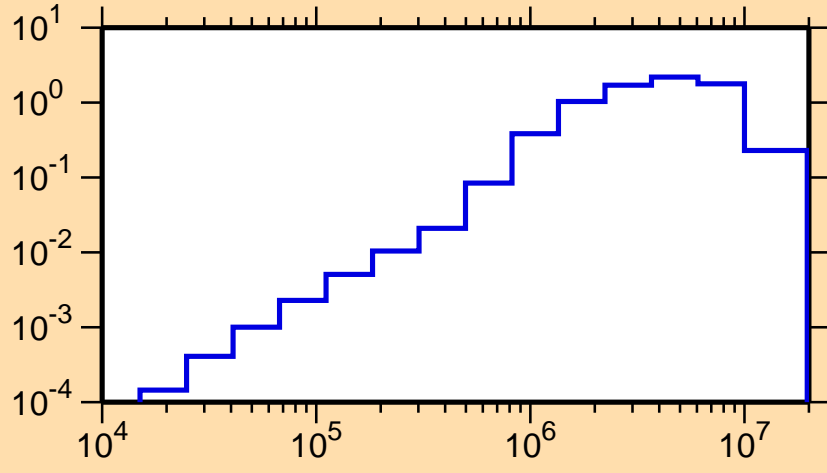
\sigma vs. E for ^{127}\text{Sn}(n,\text{inel.})
