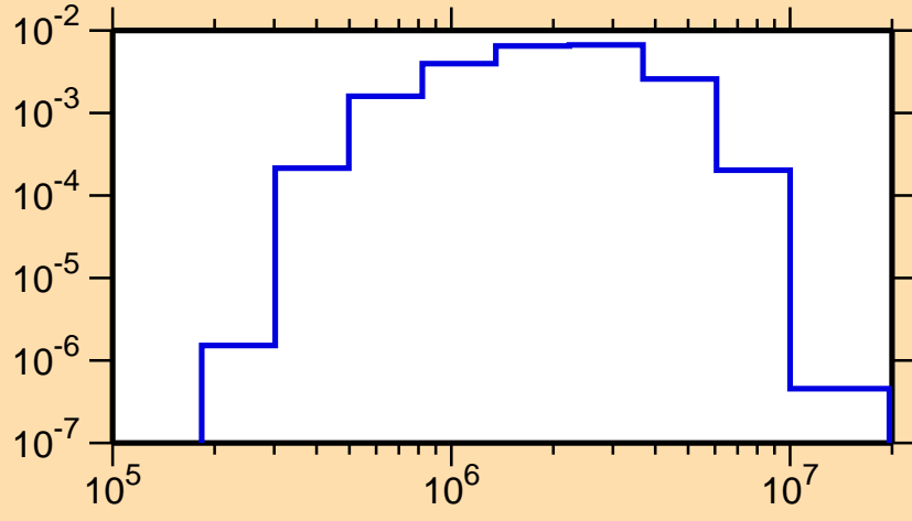
\sigma vs. E for ^{127}\text{Sn}(n,n_2)
