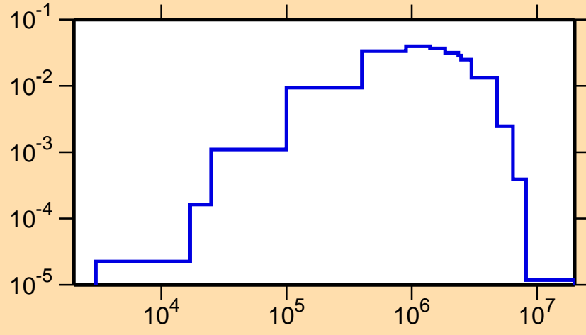
\sigma vs. E for ^{127}\text{Sn}(n,n_1)
