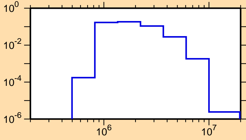
\sigma vs. E for ^{127}\text{Sn}(n,n_4)
