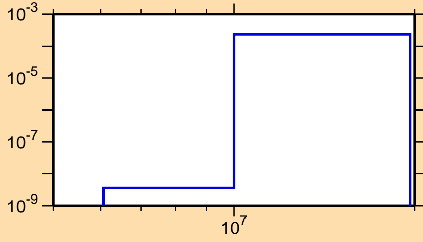
\sigma vs. E for ^{127}\text{Sn}(n,p)
