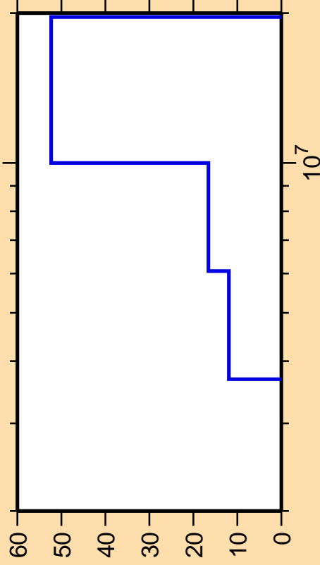
\Delta\sigma/\sigma vs. E for ^{127}\text{Sn}(n,n_{\text{cont}}) .
