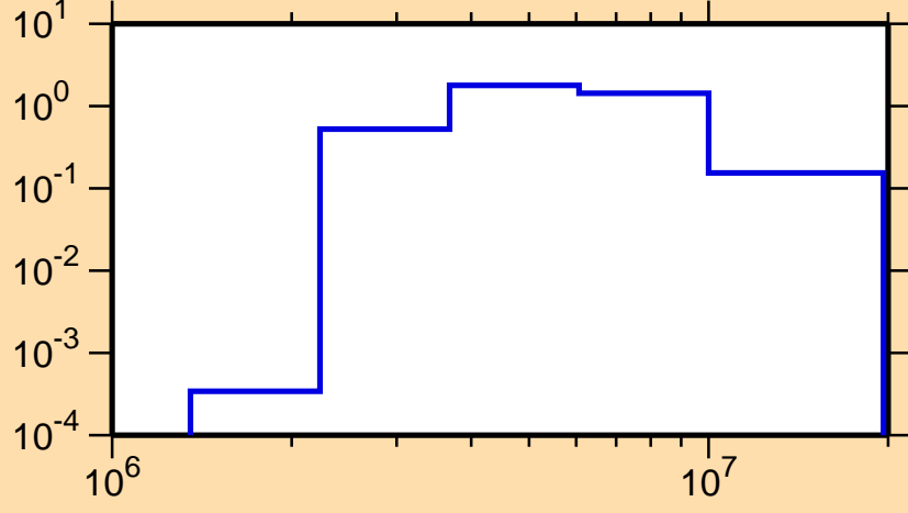
\sigma vs. E for ^{127}\text{Sn}(n,n\text{cont.})
