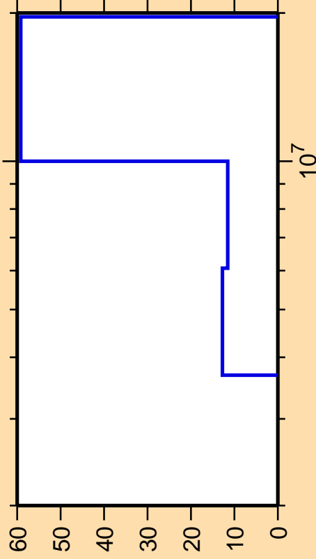
\Delta\sigma/\sigma vs. E for ^{128}\text{Sn}(n,n\text{cont.})
