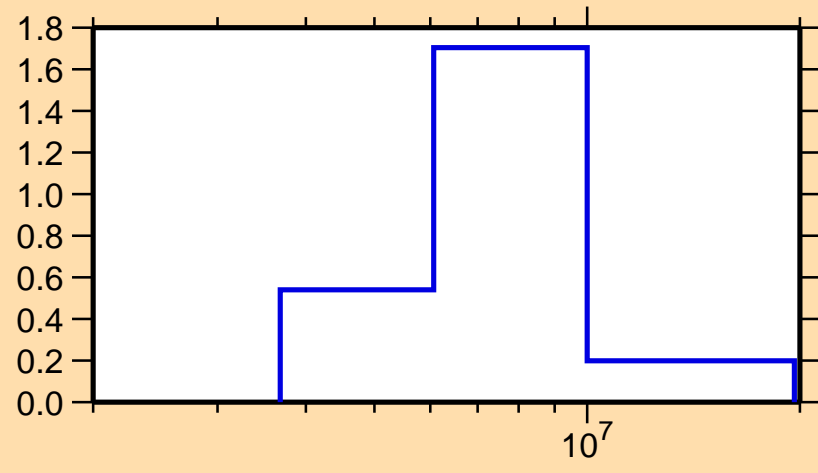
\sigma vs. E for ^{128}\text{Sn}(n,n\text{cont.})
