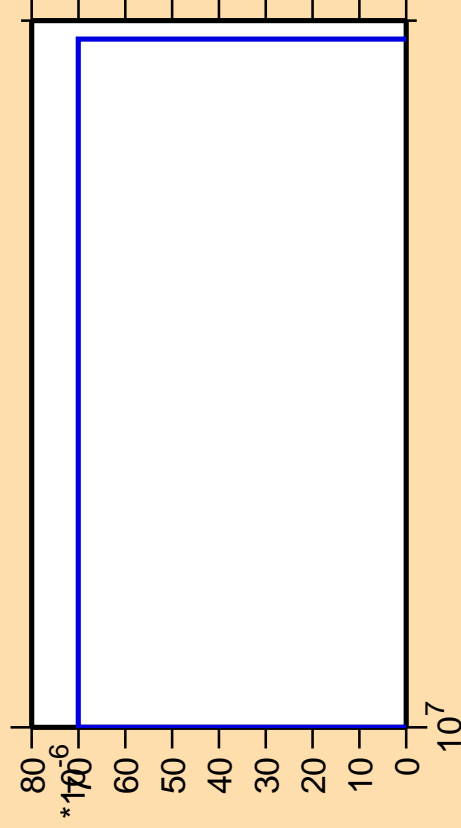
\Delta\sigma/\sigma vs. E for ^{128}\text{Sn}(n,nd)
