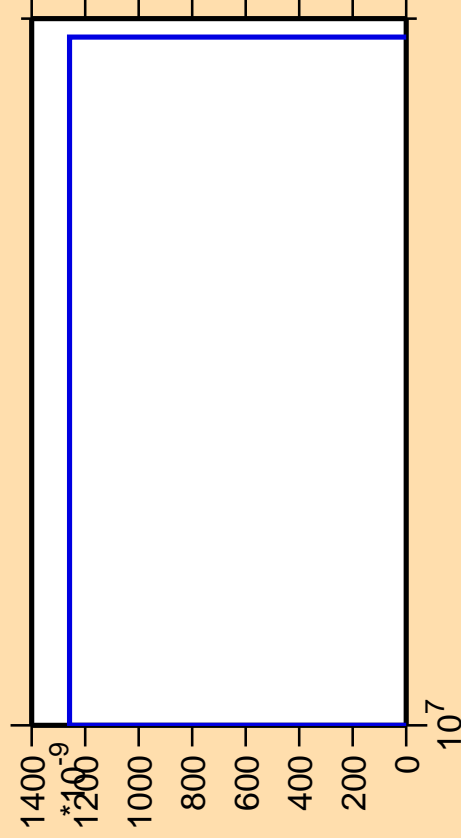
\Delta\sigma/\sigma vs. E for ^{128}\text{Sn}(n,nt)
