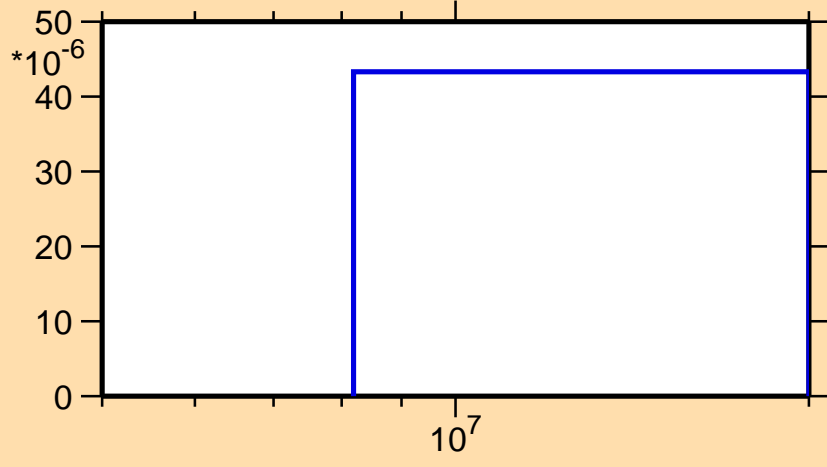
\sigma vs. E for ^{128}\text{Sn}(n,p)
