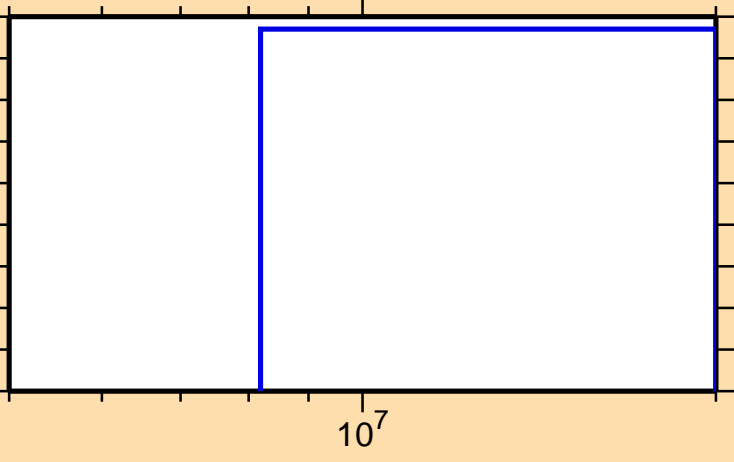
\sigma vs. E for ^{128}\text{Sn}(n,d)
