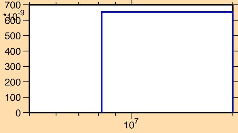
\sigma vs. E for ^{128}\text{Sn}(n,\alpha)
