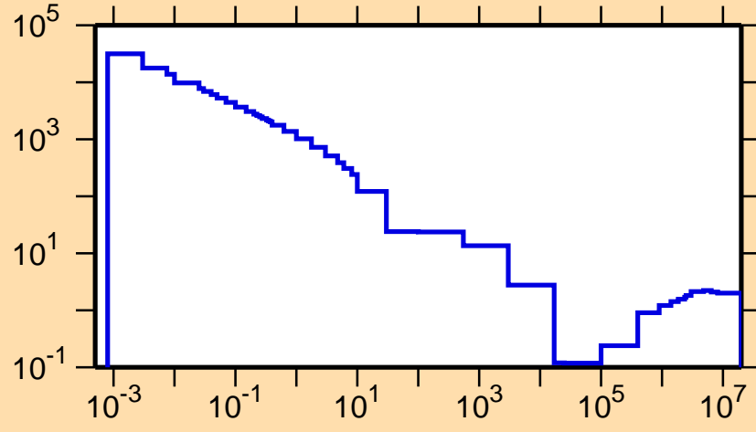
\sigma vs. E for ^{128}\text{Sn}(n,\text{nonel.})
