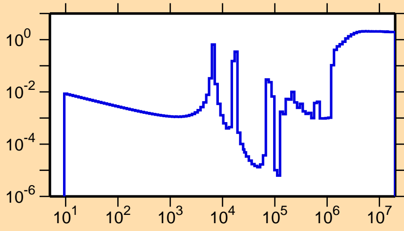
\sigma vs. E for ^{130}\text{Sn}(n,\text{nonel.})
