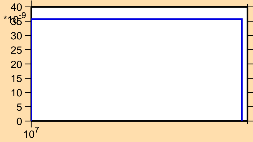
\sigma vs. E for ^{130}\text{Sn}(n,d)
