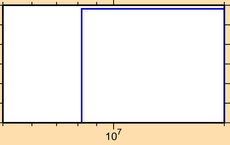
\sigma vs. E for ^{131}\text{Sn}(n,t)
