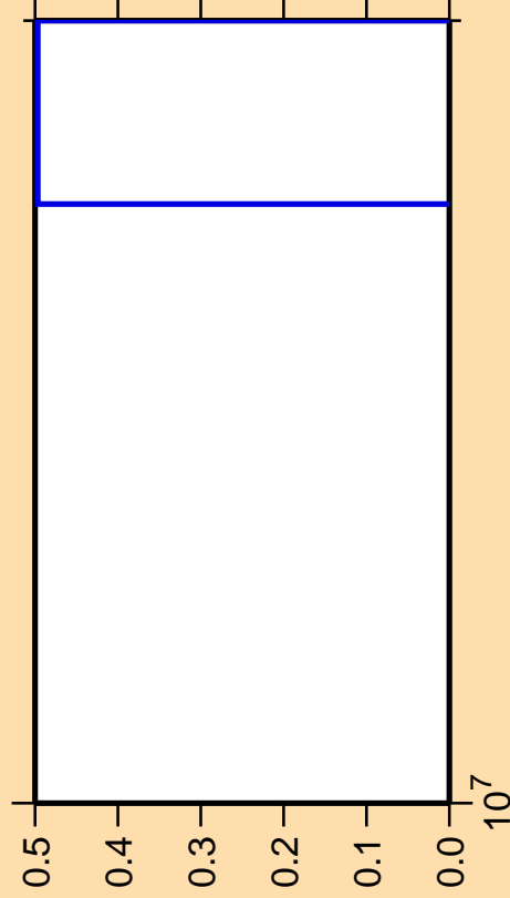
\Delta\sigma/\sigma vs. E for ^{131}\text{Sn}(n,\text{nd})
