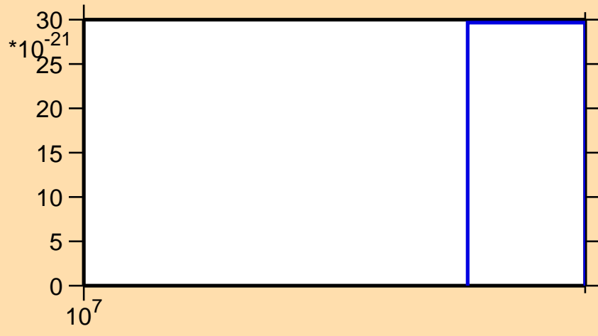
\sigma vs. E for ^{131}\text{Sn}(n,2np)
