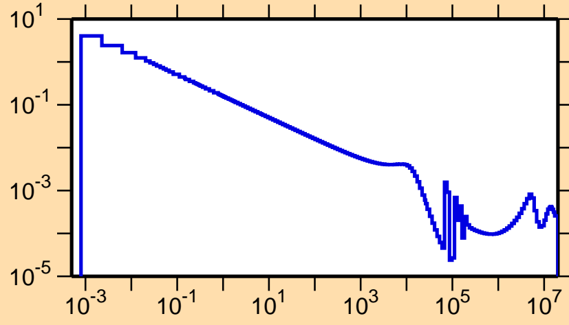
\sigma vs. E for ^{131}\text{Sn}(n,\gamma)
