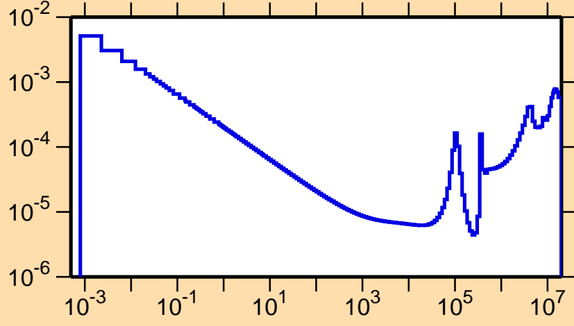
\sigma vs. E for ^{132}\text{Sn}(n,\gamma)
