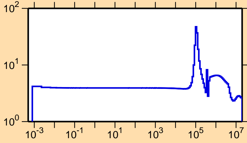
\sigma vs. E for ^{132}\text{Sn}(n,\text{el.})
