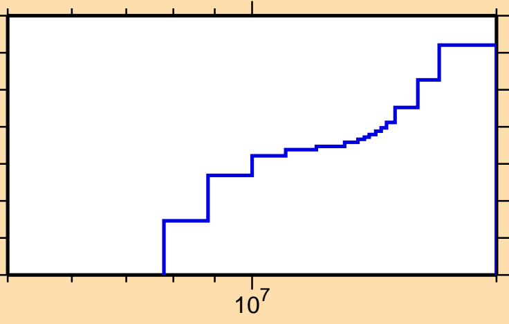
\sigma vs. E for ^{132}\text{Sn}(n,n\text{cont.})
