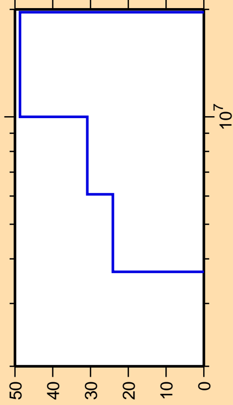
\Delta\sigma/\sigma vs. E for ^{132}\text{Sn}(n,n_4)
