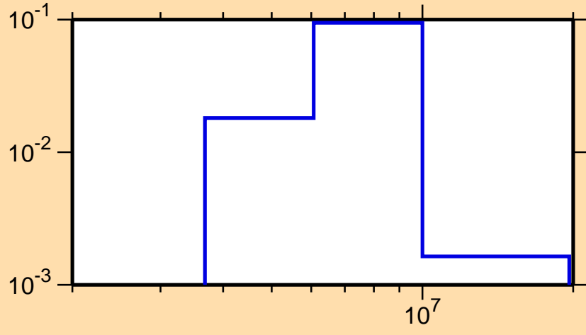
\sigma vs. E for ^{132}\text{Sn}(n,n_4)
