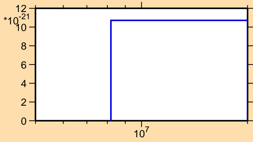
\sigma vs. E for ^{132}\text{Sn}(n,nd)
