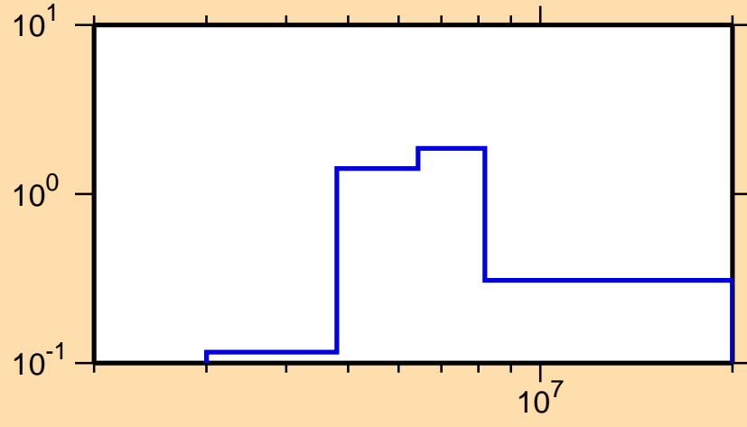
\sigma vs. E for ^{132}\text{Sn}(n,\text{inel.})
