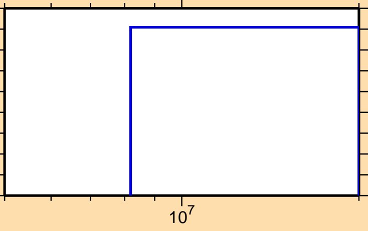
\sigma vs. E for ^{132}\text{Sn}(n,n\alpha)
