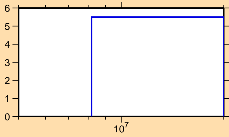
\Delta\sigma/\sigma vs. E for ^{132}\text{Sn}(n,\text{tot.})
