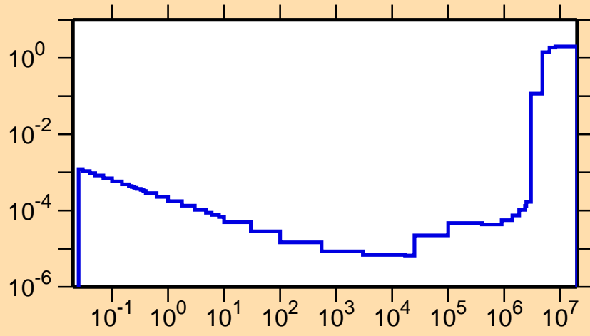
\sigma vs. E for ^{132}\text{Sn}(n,\text{nonel.})
