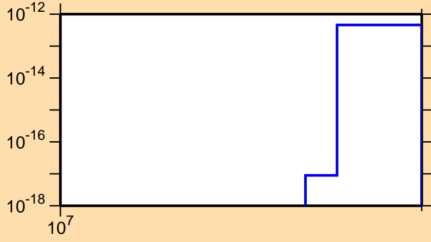
\sigma vs. E for ^{133}\text{Sn}(n,\text{nd})
