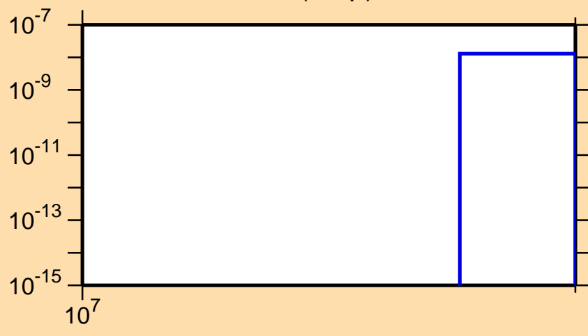
\sigma vs. E for ^{133}\text{Sn}(n,np)
