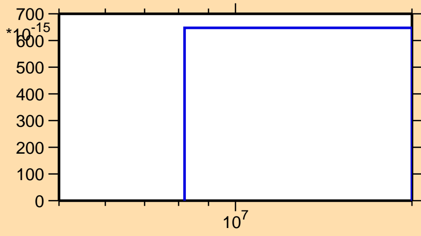
\sigma vs. E for ^{133}\text{Sn}(n,nt)
