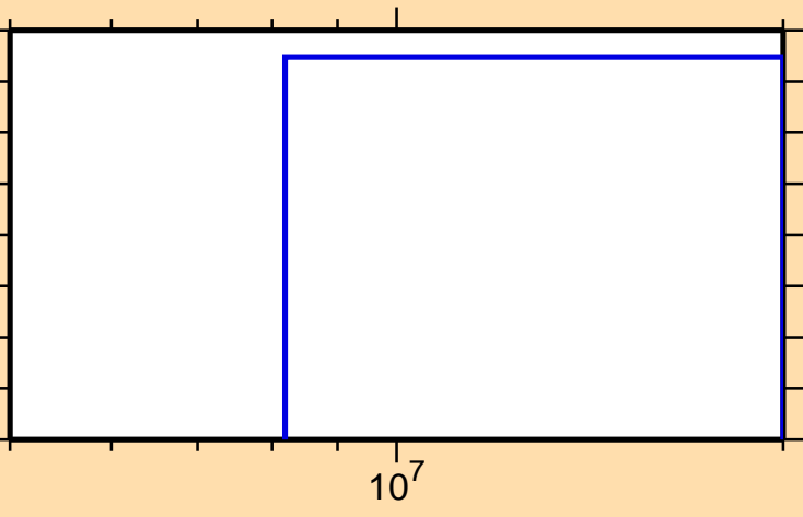
\sigma vs. E for ^{133}\text{Sn}(n,nd)
