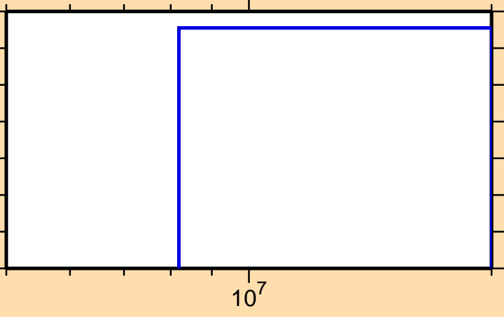
\sigma vs. E for ^{133}\text{Sn}(n,\alpha)
