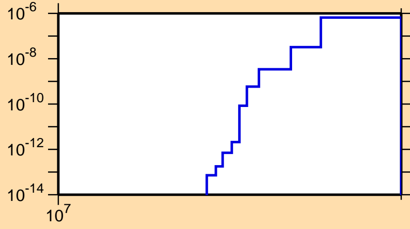
\sigma vs. E for ^{76}\text{Sr} (mt 45)
