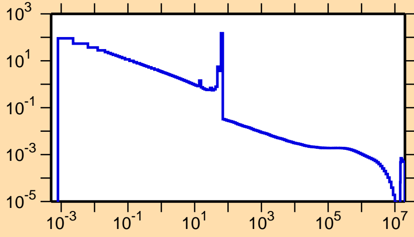
\sigma vs. E for ^{76}\text{Sr}(n,\gamma)
