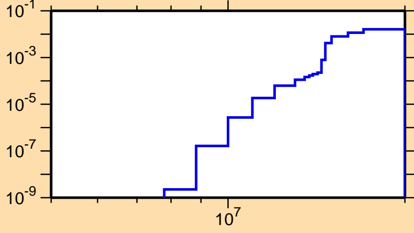
\sigma vs. E for ^{76}\text{Sr}(n,pd)
