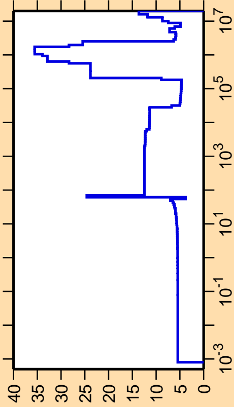
\Delta\sigma/\sigma vs. E for ^{76}\text{Sr}(n,\text{el.})
