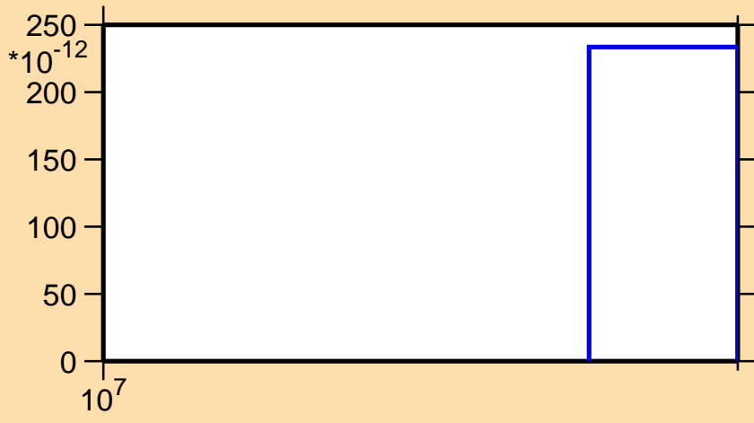
\sigma vs. E for ^{76}\text{Sr}(n,2np)
