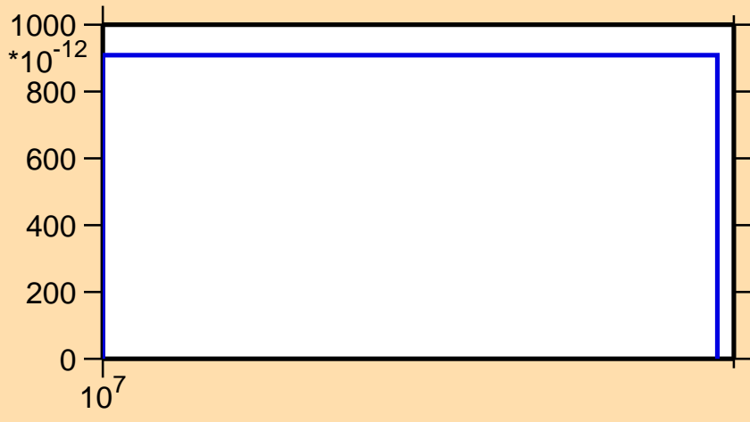
\sigma vs. E for ^{76}\text{Sr}(\text{mt117})
