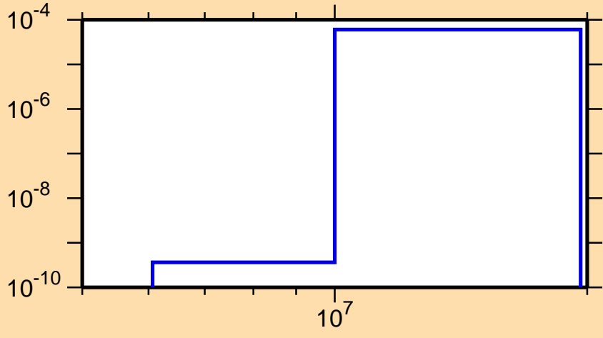
\sigma vs. E for ^{76}\text{Sr}(n,\alpha)
