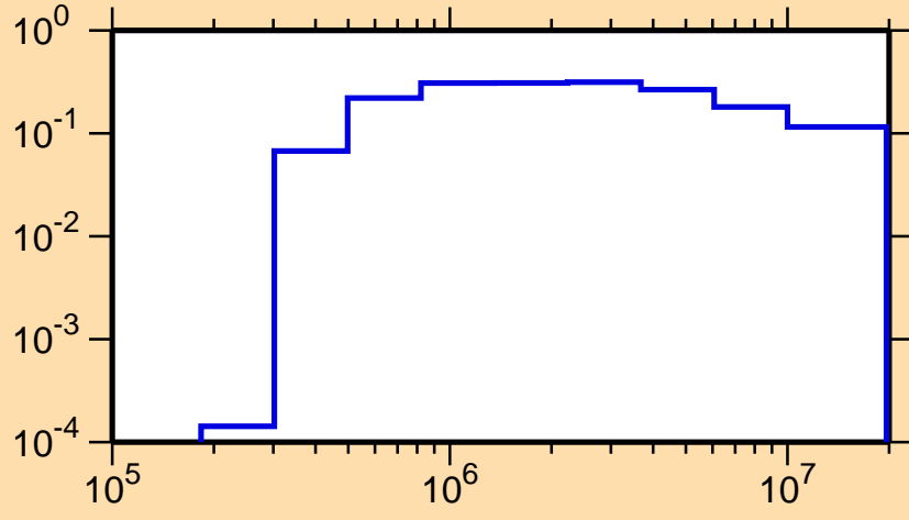
\sigma vs. E for ^{76}\text{Sr}(n,n_1)
