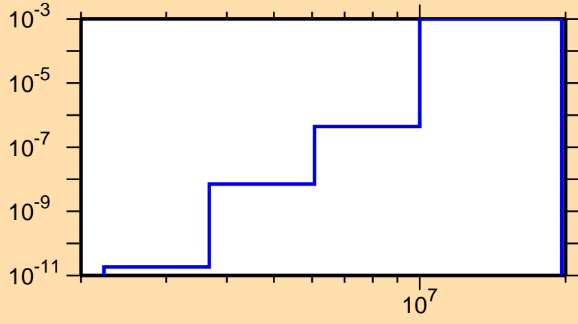
\sigma vs. E for ^{76}\text{Sr}(n,\text{He}3)
