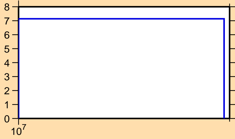
\Delta\sigma/\sigma vs. E for ^{76}\text{Sr}(n,\text{tot.})
