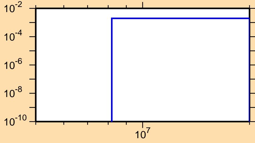
\sigma vs. E for ^{76}\text{Sr}(n,\text{pd})
