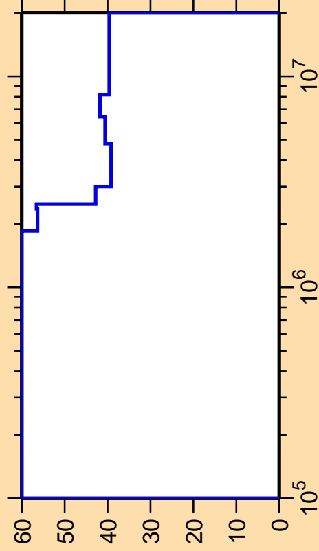
\Delta\sigma/\sigma vs. E for ^{76}\text{Sr}(n,\text{inel.})
