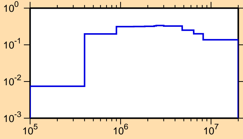
\sigma vs. E for ^{76}\text{Sr}(n,\text{inel.})
