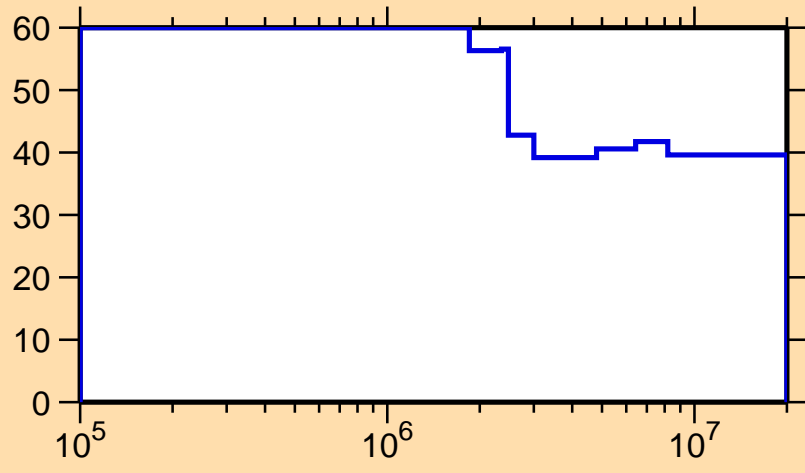
\Delta\sigma/\sigma vs. E for ^{76}\text{Sr}(n,\text{inel.})
