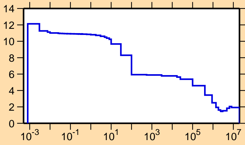
\sigma vs. E for ^{76}\text{Sr}(n,\text{el.})
