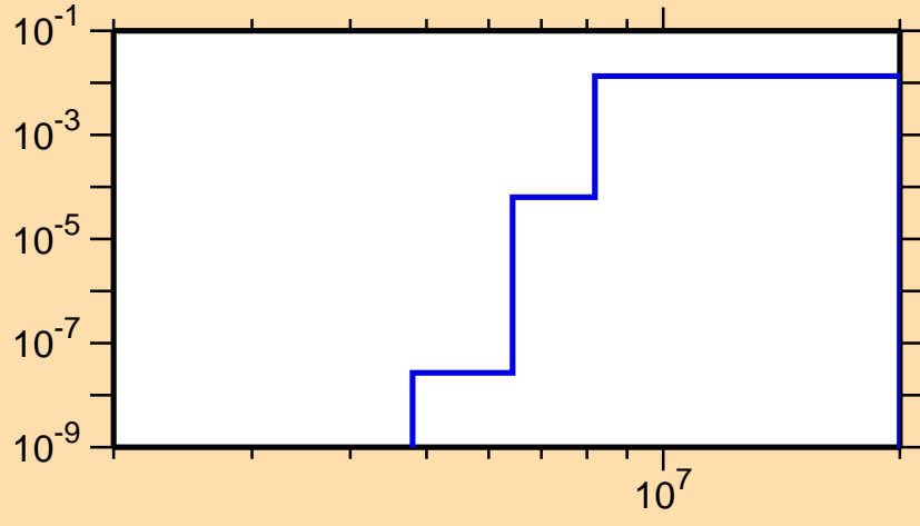
\sigma vs. E for ^{76}\text{Sr}(n,np)
