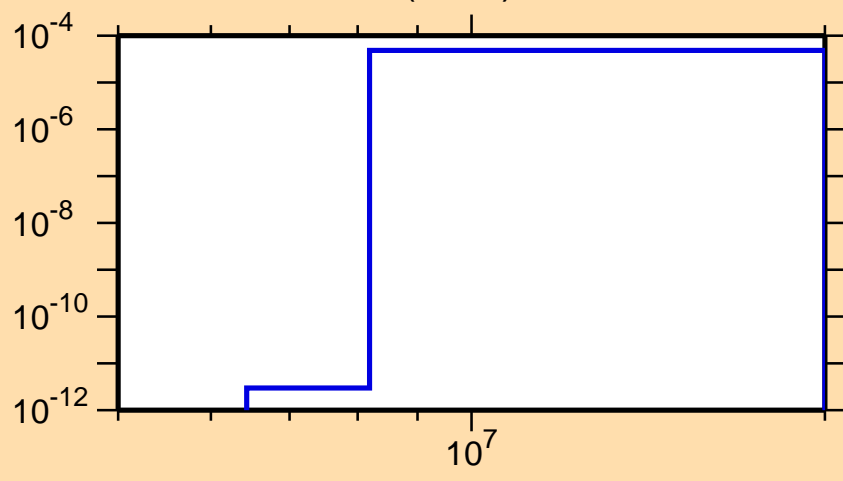
\sigma vs. E for ^{76}\text{Sr}(n,n\alpha)
