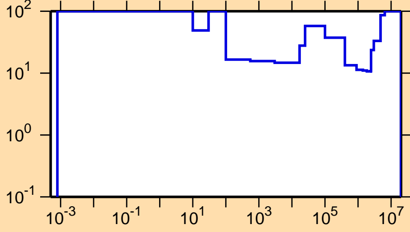
\Delta\sigma/\sigma vs. E for ^{76}\text{Sr}(n,p)
