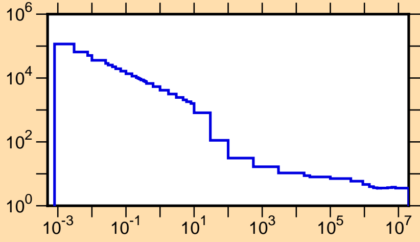
\sigma vs. E for ^{76}\text{Sr}(n,\text{tot.})
