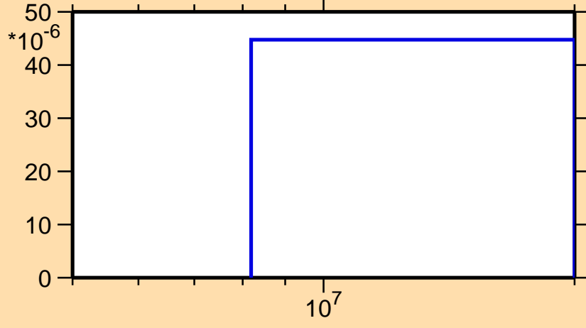
\sigma vs. E for ^{76}\text{Sr}(n,t)
