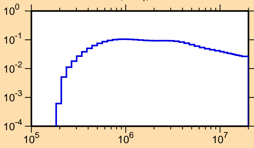
\sigma vs. E for ^{77}\text{Sr}(n,n_1)
