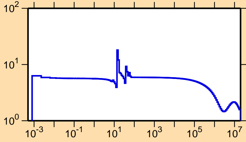
\sigma vs. E for ^{77}\text{Sr}(n,\text{el.})
