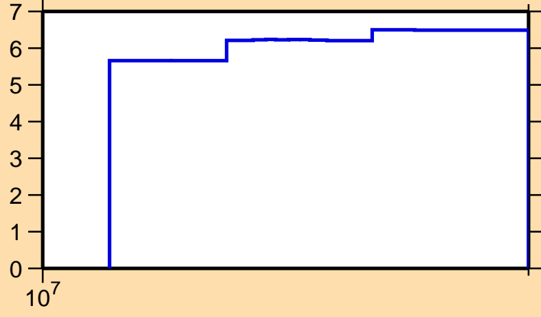
\Delta\sigma/\sigma vs. E for ^{77}\text{Sr}(n,\text{nonel.})
