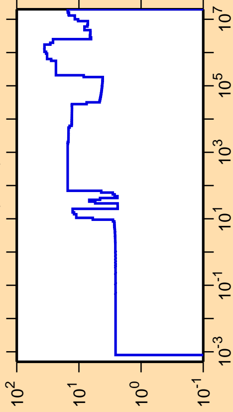
\Delta\sigma/\sigma vs. E for ^{77}\text{Sr}(n,\text{el.})
