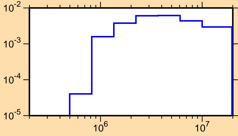
\sigma vs. E for ^{77}\text{Sr}(n,n_4)
