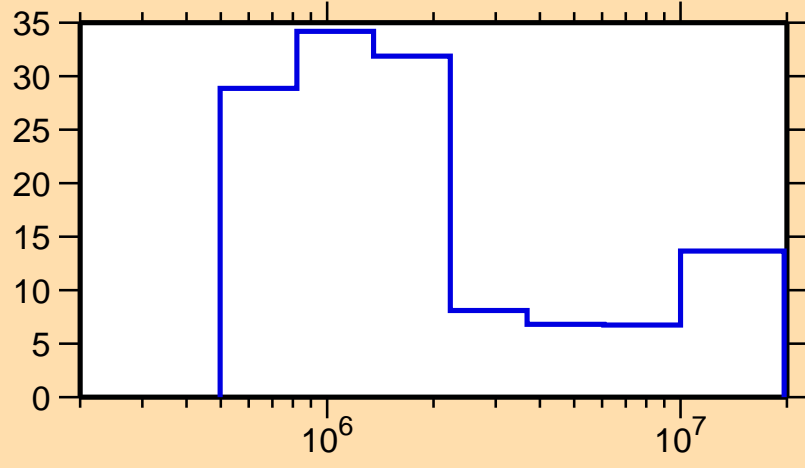
\Delta\sigma/\sigma vs. E for ^{77}\text{Sr}(n,el.)
