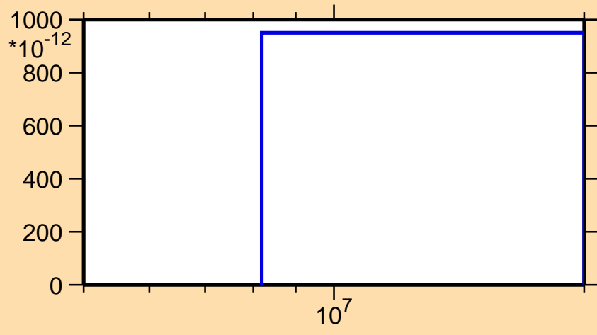
\sigma vs. E for ^{77}\text{Sr}(\text{mt } 45)
