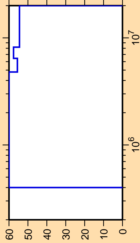
\Delta\sigma/\sigma vs. E for ^{77}\text{Sr}(n,n_2)
