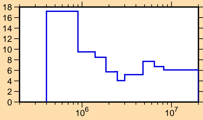
\Delta\sigma/\sigma vs. E for ^{77}\text{Sr}(n,n\text{onel.})
