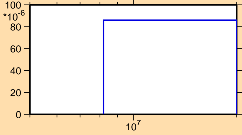
\sigma vs. E for ^{77}\text{Sr}(n,t)
