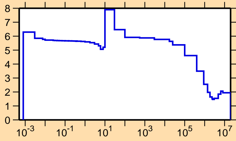
\sigma vs. E for ^{77}\text{Sr}(n,\text{el.})
