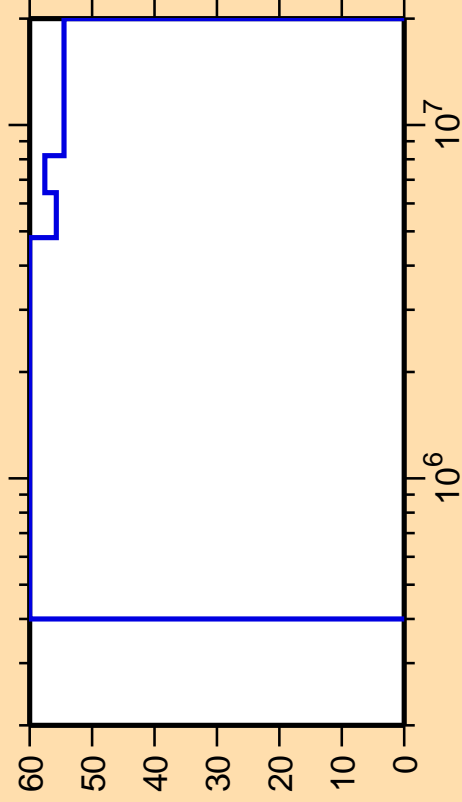
\Delta\sigma/\sigma vs. E for ^{77}\text{Sr}(n,n_3)
