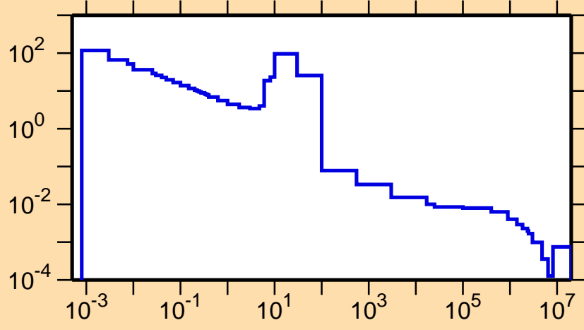
\sigma vs. E for ^{77}\text{Sr}(n,\gamma)
