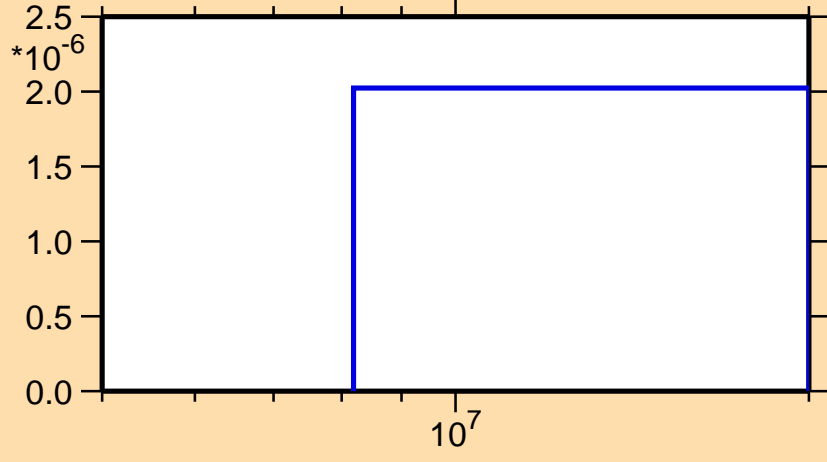
\sigma vs. E for ^{77}\text{Sr}(n,\text{pt})
