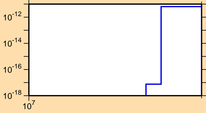
\sigma vs. E for ^{78}\text{Sr} (mt 34)
