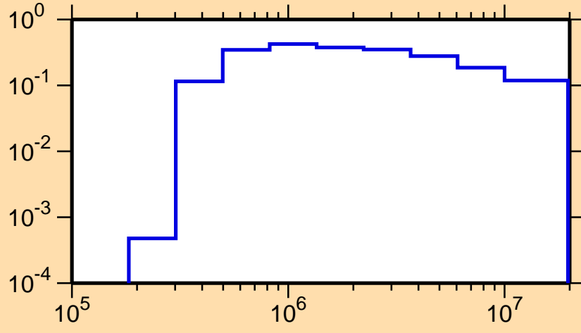
\sigma vs. E for ^{78}\text{Sr}(n,n_1)
