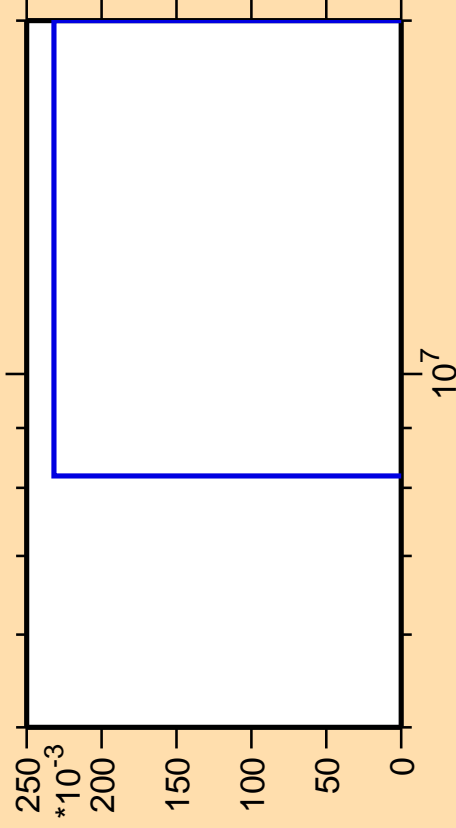
\Delta\sigma/\sigma vs. E for ^{78}\text{Sr}(n,2np)
