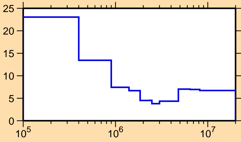
\Delta\sigma/\sigma vs. E for ^{78}\text{Sr}(n,\text{nonel.})
