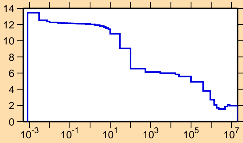
\sigma vs. E for ^{78}\text{Sr}(n,\text{el.})
