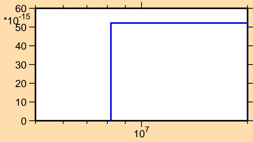
\sigma vs. E for ^{78}\text{Sr}(\text{mt } 34)
