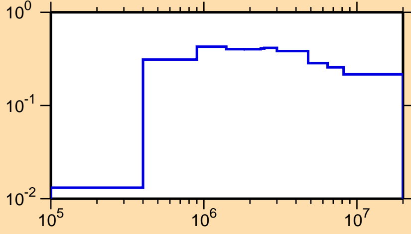
\sigma vs. E for ^{78}\text{Sr}(n,\text{inel.})
