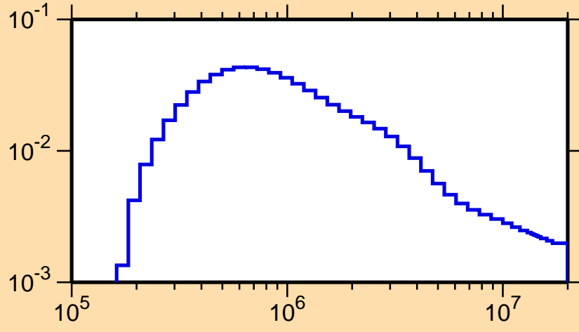
\sigma vs. E for ^{79}\text{Sr}(n,n_1)
