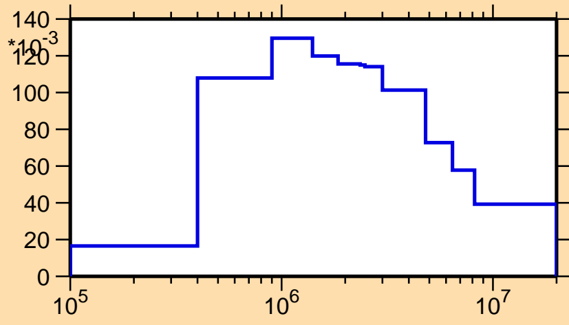
\sigma vs. E for ^{79}\text{Sr}(n,n_2)
