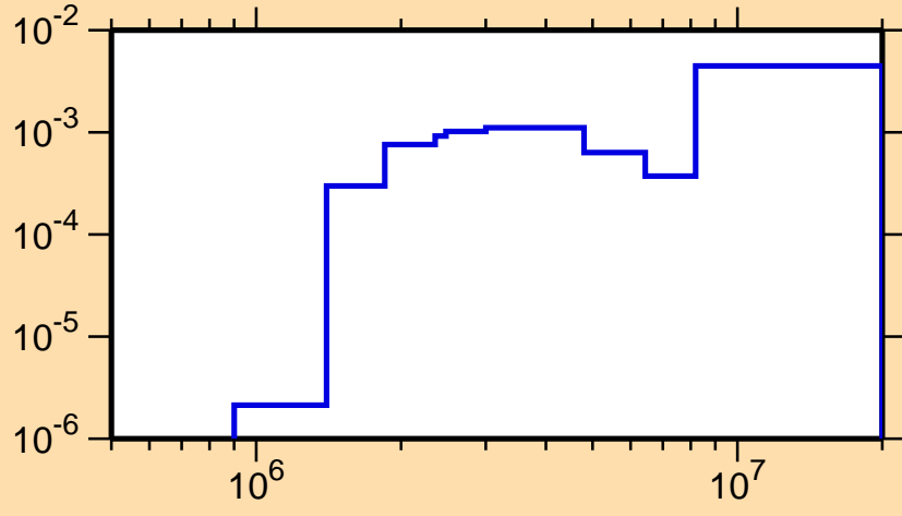
\sigma vs. E for ^{79}\text{Sr}(n,n\text{cont.})
