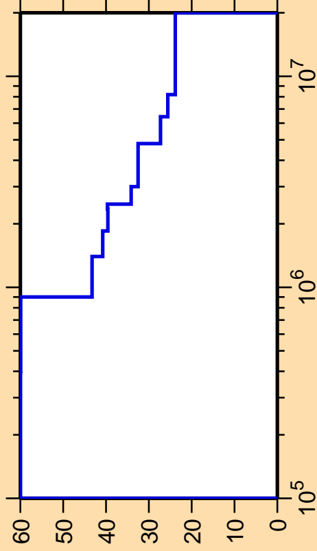
\Delta\sigma/\sigma vs. E for ^{79}\text{Sr}(n,n_2)
