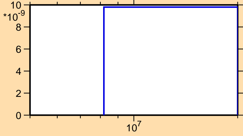
\sigma vs. E for ^{79}\text{Sr}(n,\text{nd})
