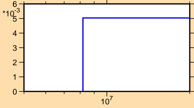
\sigma vs. E for ^{79}\text{Sr}(n,2n)
