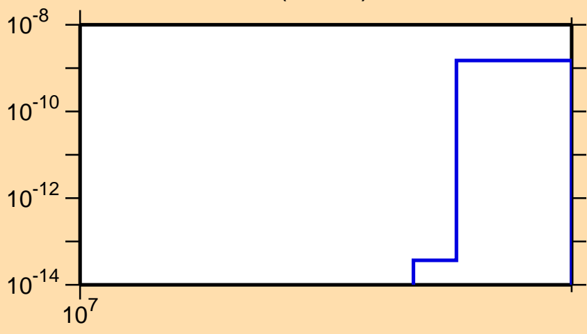
\sigma vs. E for ^{80}\text{Sr} (mt 45)
