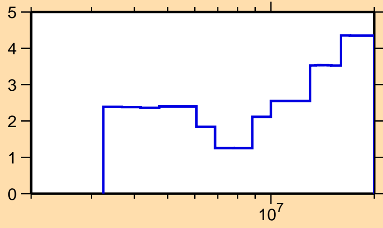
\Delta\sigma/\sigma vs. E for ^{80}\text{Sr}(n,\text{tot.})
