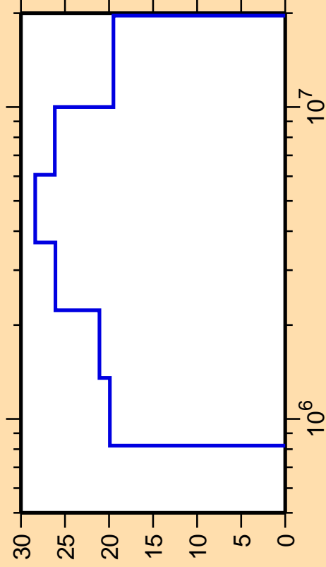
\Delta\sigma/\sigma vs. E for ^{80}\text{Sr}(n,n_3)
