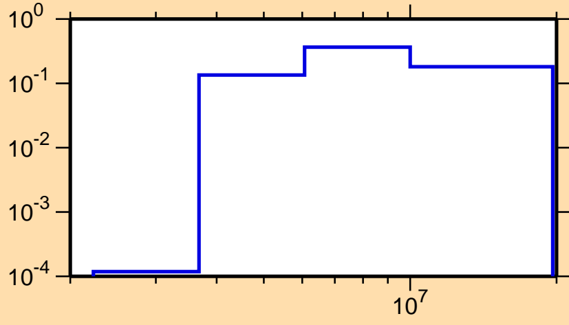
\sigma vs. E for ^{80}\text{Sr}(n,n\text{cont.})
