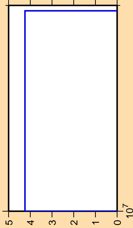
\Delta\sigma/\sigma vs. E for ^{80}\text{Sr} (mt117)
