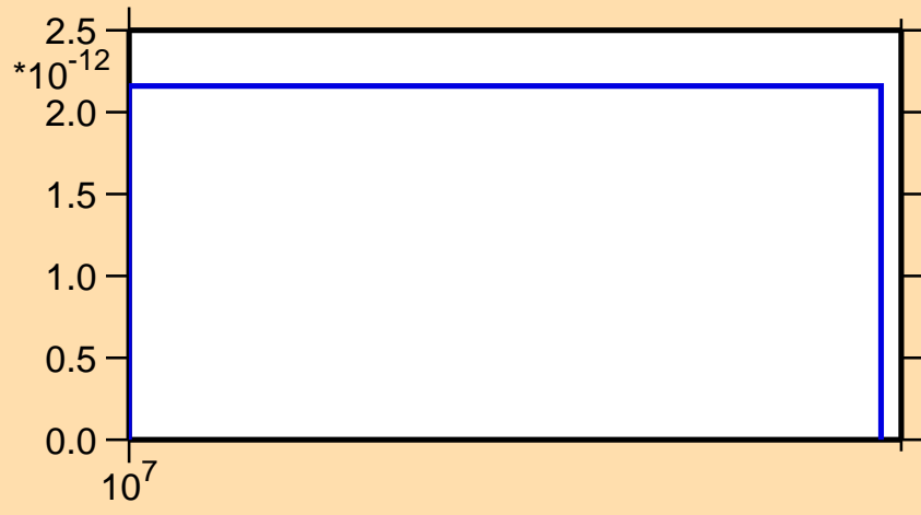
\sigma vs. E for ^{80}\text{Sr} (mt117)
