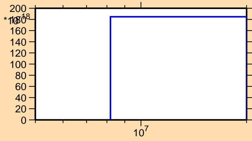
\sigma vs. E for ^{80}\text{Sr}(n,2np)
