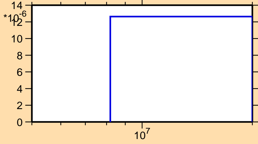
\sigma vs. E for ^{80}\text{Sr}(n,\text{pd})
