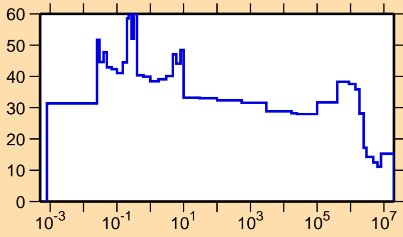
\Delta\sigma/\sigma vs. E for ^{80}\text{Sr}(n,p)
