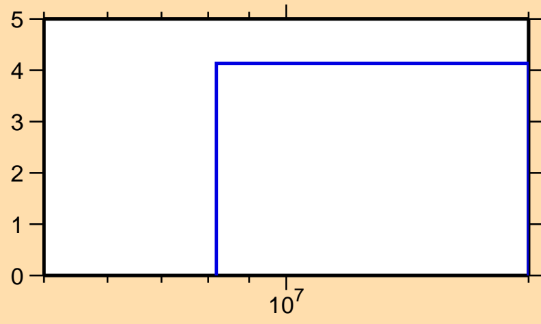
\Delta\sigma/\sigma vs. E for ^{80}\text{Sr}(n,\text{nonel.})
