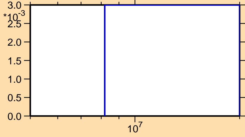
\sigma vs. E for ^{80}\text{Sr}(n,2n)
