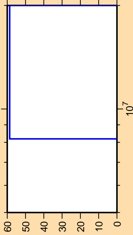
\Delta\sigma/\sigma vs. E for ^{80}\text{Sr}(n,2n)
