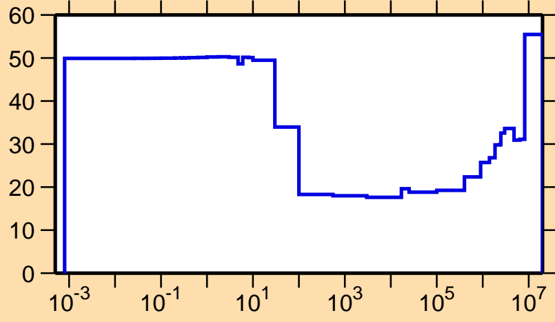
\Delta\sigma/\sigma vs. E for ^{80}\text{Sr}(n,\gamma)
