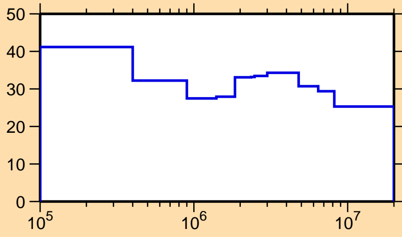
\Delta\sigma/\sigma vs. E for ^{80}\text{Sr}(n,n_1)
