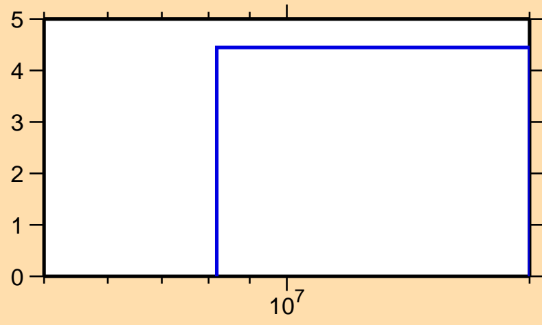
\Delta\sigma/\sigma vs. E for ^{80}\text{Sr}(n,\text{el.})
