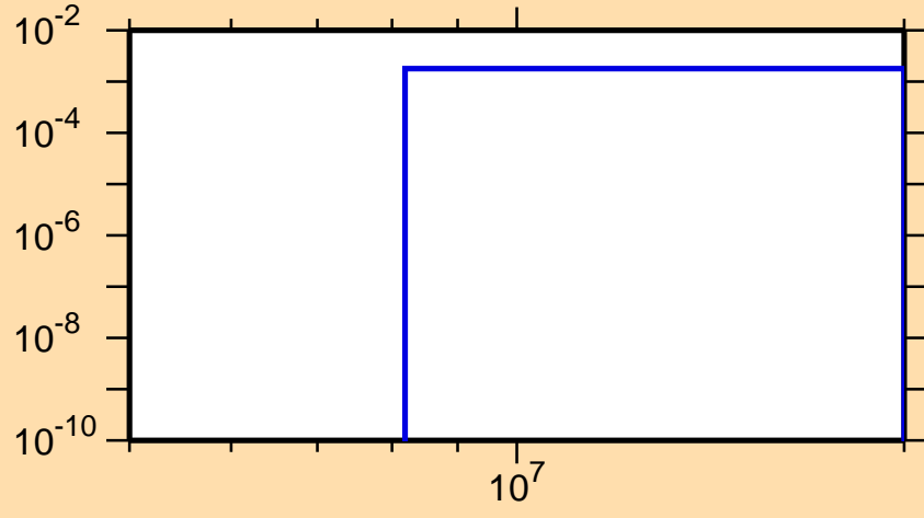
\sigma vs. E for ^{80}\text{Sr}(n,p\alpha)
