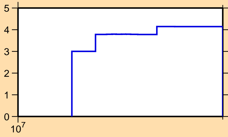
\Delta\sigma/\sigma vs. E for ^{82}\text{Sr}(n,\text{tot.})
