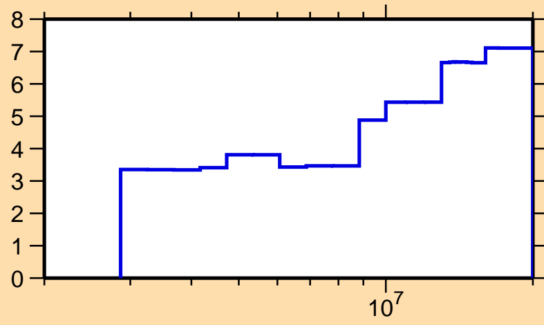
\Delta\sigma/\sigma vs. E for ^{82}\text{Sr}(n,el.)
