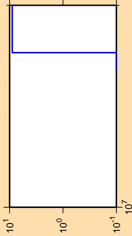
\Delta\sigma/\sigma vs. E for ^{82}\text{Sr} (mt117)
