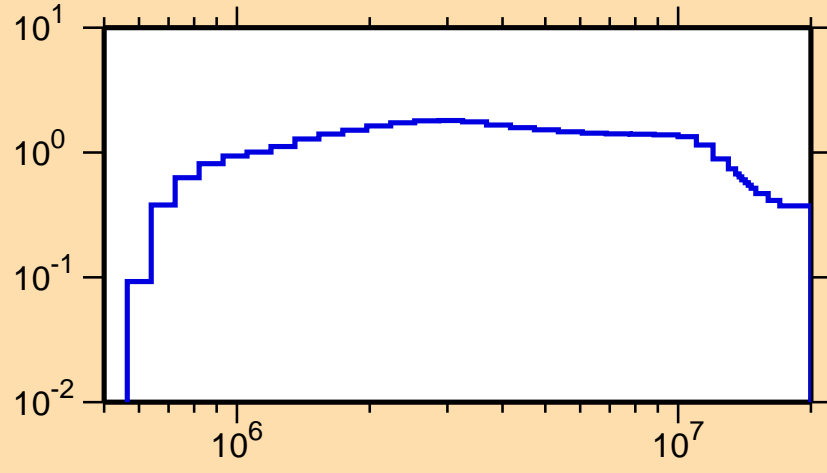
\sigma vs. E for ^{82}\text{Sr}(n,\text{inel.})
