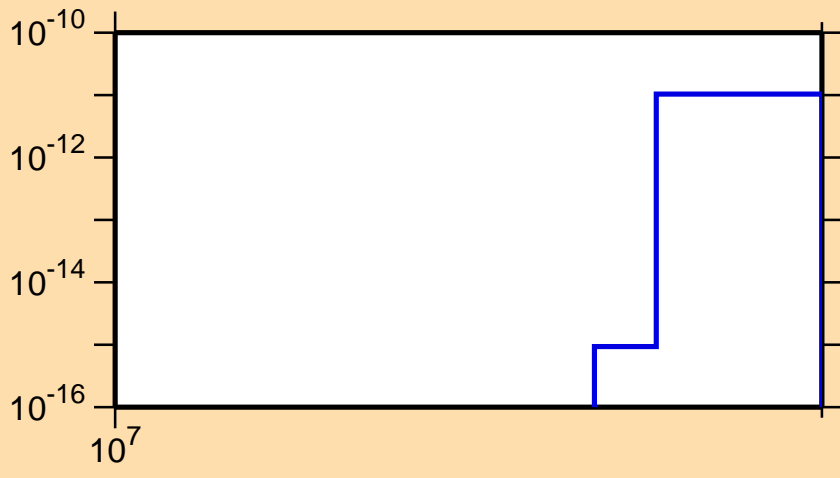
\sigma vs. E for ^{82}\text{Sr} (mt117)
