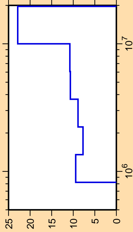
\Delta\sigma/\sigma vs. E for ^{82}\text{Sr}(n,n_2)
