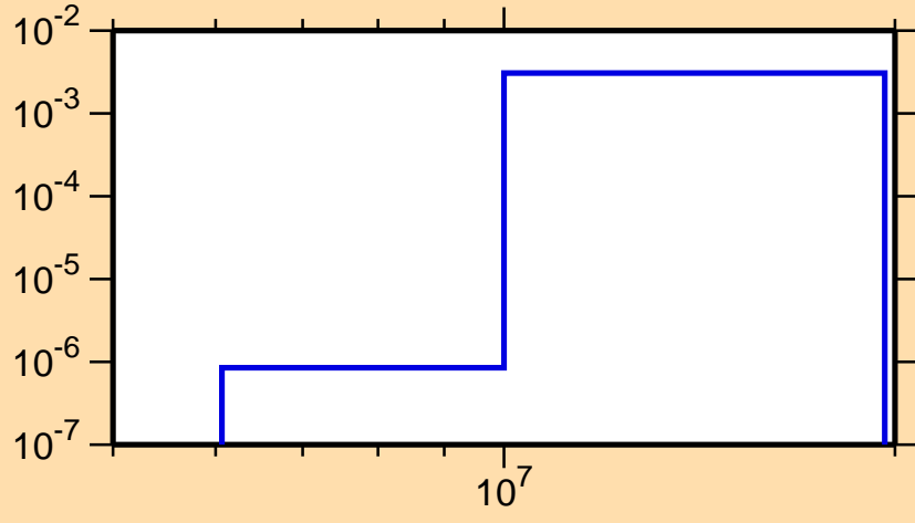
\sigma vs. E for ^{82}\text{Sr}(n,d)
