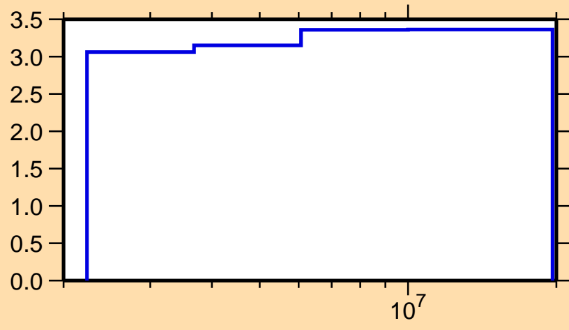
\Delta\sigma/\sigma vs. E for ^{82}\text{Sr}(n,n\text{onel.})
