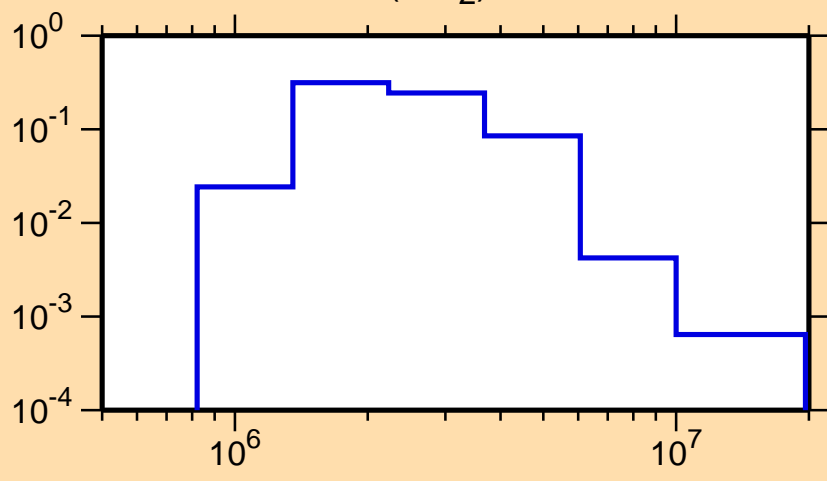
\sigma vs. E for ^{82}\text{Sr}(n,n_2)
