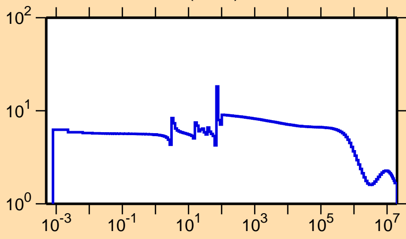
\sigma vs. E for ^{83}\text{Sr}(n,\text{el.})
