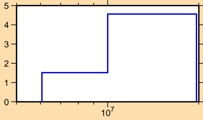
\Delta\sigma/\sigma vs. E for ^{83}\text{Sr}(n,\text{el.})
