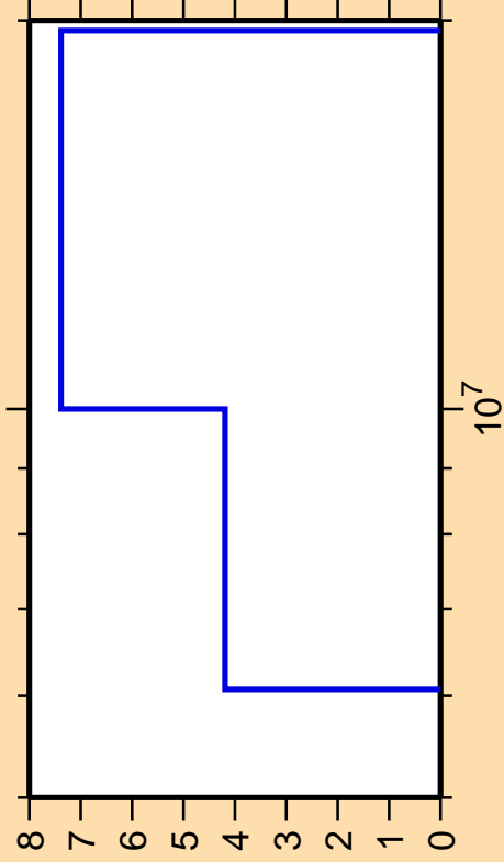
\Delta\sigma/\sigma vs. E for ^{83}\text{Sr}(n,n_{\text{cont}})
