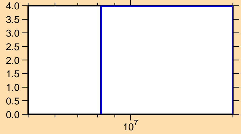
\Delta\sigma/\sigma vs. E for ^{83}\text{Sr}(n,\text{el.})
