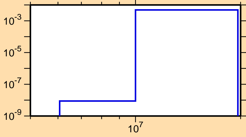
\sigma vs. E for ^{83}\text{Sr}(n,\alpha)
