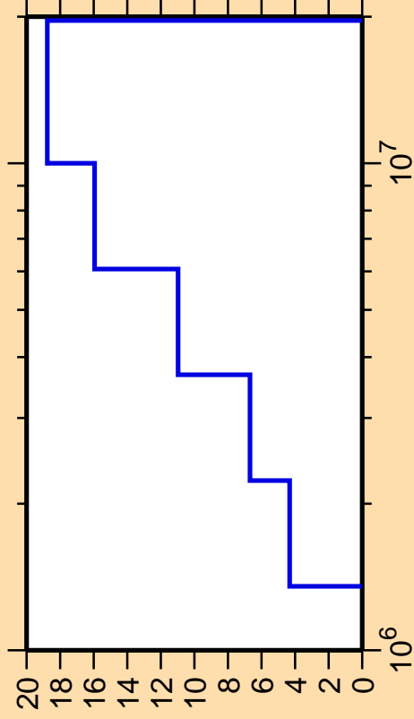
\Delta\sigma/\sigma vs. E for ^{84}\text{Sr}(n,n_3)
