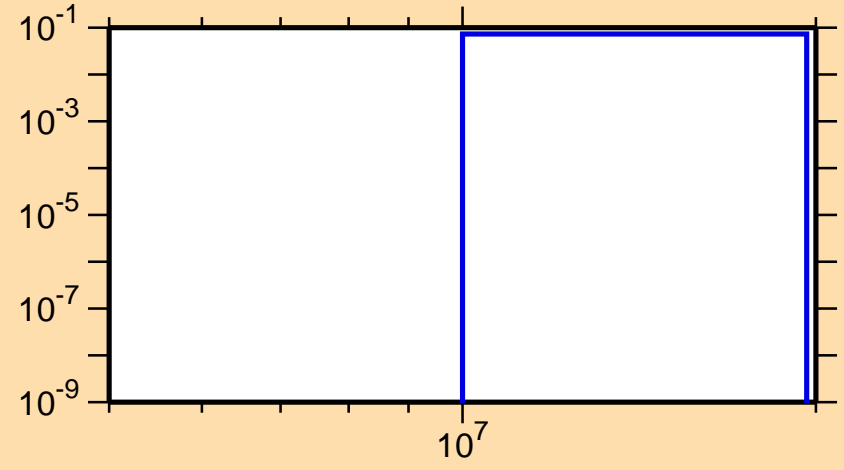
\sigma vs. E for ^{84}\text{Sr}(n,np)
