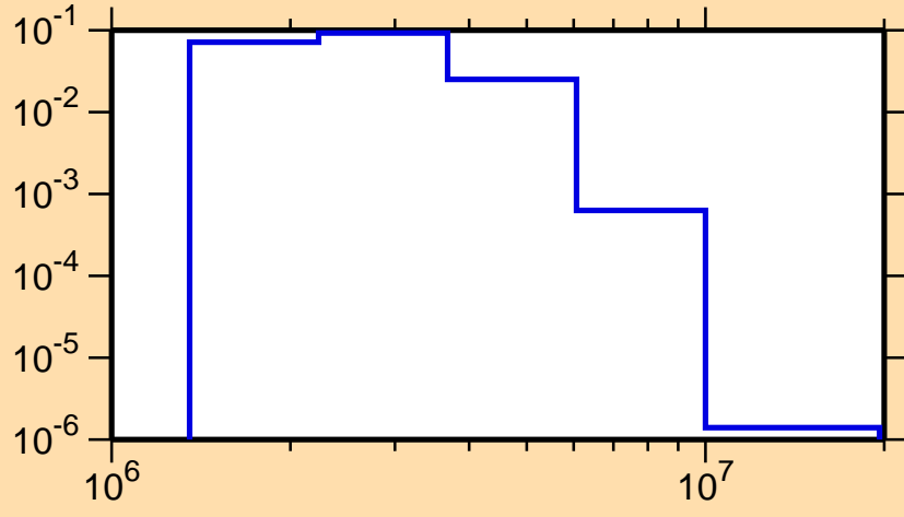
\sigma vs. E for ^{84}\text{Sr}(n,n_3)
