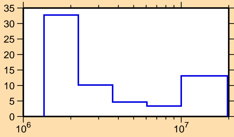
\Delta\sigma/\sigma vs. E for ^{85}\text{Sr}(n,n\text{cont.})
