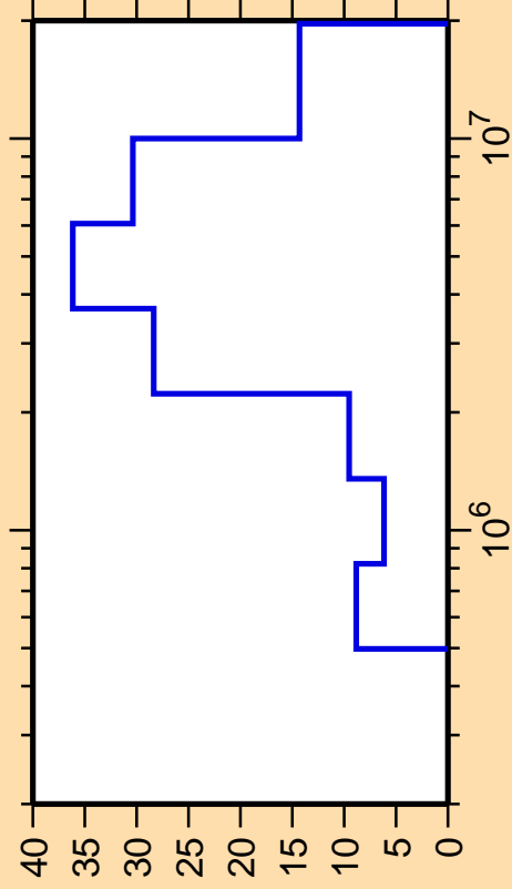
\Delta\sigma/\sigma vs. E for ^{85}\text{Sr}(n,n_3)
