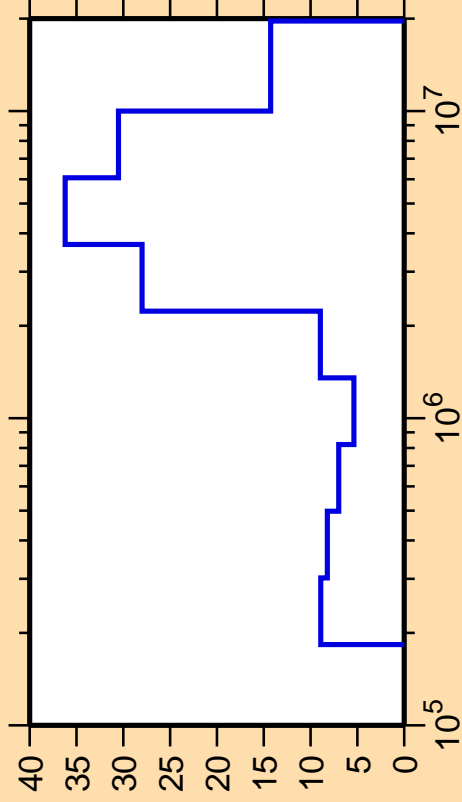
\Delta\sigma/\sigma vs. E for ^{85}\text{Sr}(n,n_2)
