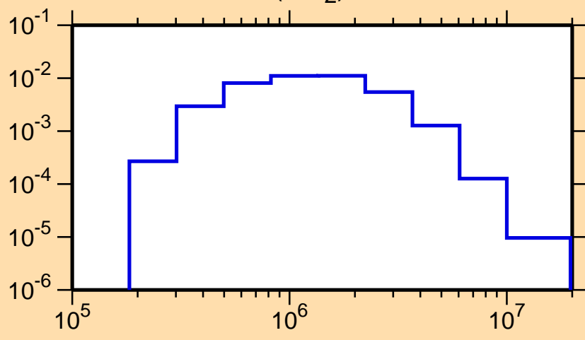
\sigma vs. E for ^{85}\text{Sr}(n,n_2)
