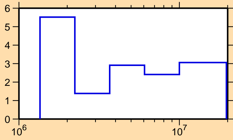
\Delta\sigma/\sigma vs. E for ^{85}\text{Sr}(n, el.)
