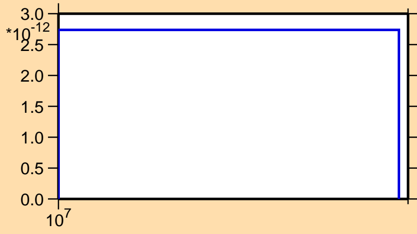
\sigma vs. E for ^{85}\text{Sr}(n,\text{pd})
