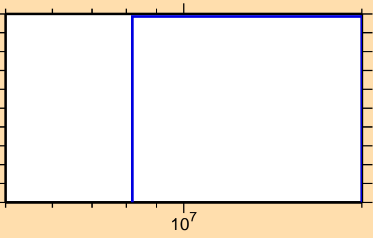
\sigma vs. E for ^{85}\text{Sr}(n,p\alpha)
