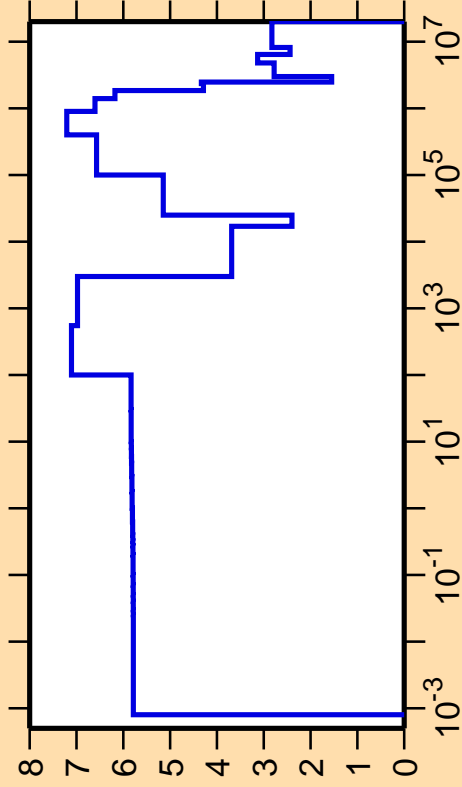
\Delta\sigma/\sigma vs. E for ^{85}\text{Sr}(n,\text{el.})
