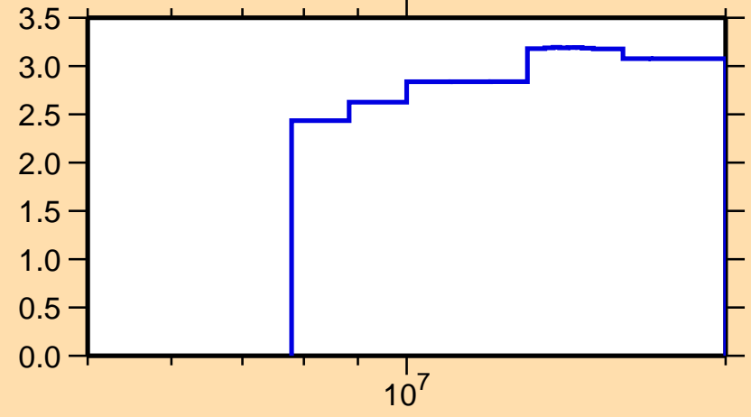
\Delta\sigma/\sigma vs. E for ^{85}\text{Sr}(n,\text{el.})
