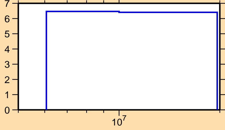
\Delta\sigma/\sigma vs. E for ^{85}\text{Sr}(n,2n)
