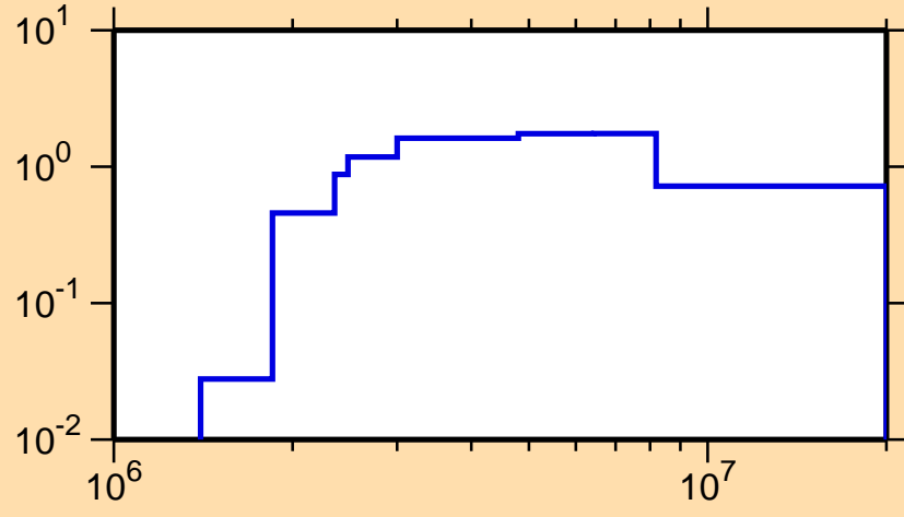
\sigma vs. E for ^{85}\text{Sr}(n,n\text{cont.})
