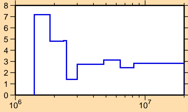
\Delta\sigma/\sigma vs. E for ^{85}\text{Sr}(n,\text{el.})
